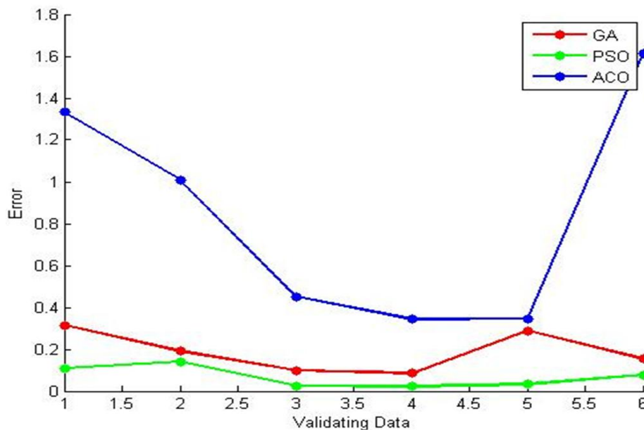
FIGURE 6 ERROR GRAPH FOR COST PERFORMANCE WITH DIFFERENT ALGORITHMS OF EXTERNAL DATA SOURCE
