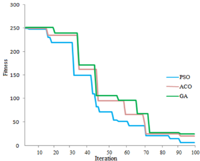
FIGURE 7 CONVERGENCE GRAPH
