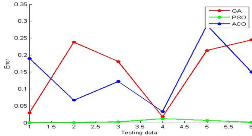
FIGURE 3 ERROR GRAPH FOR TIME PERFORMANCE WITH DIFFERENT ALGORITHMS OF SAME SOURCE DATA
