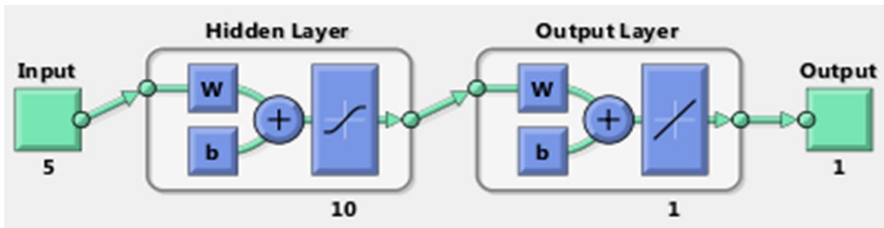
FIGURE 1 ARTIFICIAL NEURAL NETWORK STRUCTURE
